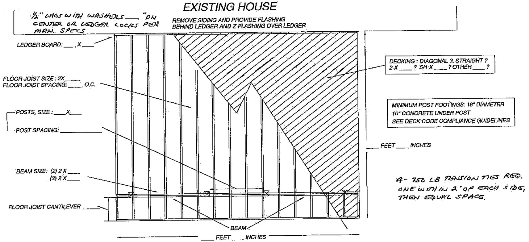
DECK FLOOR FRAMING PLAN EXAMPLE
